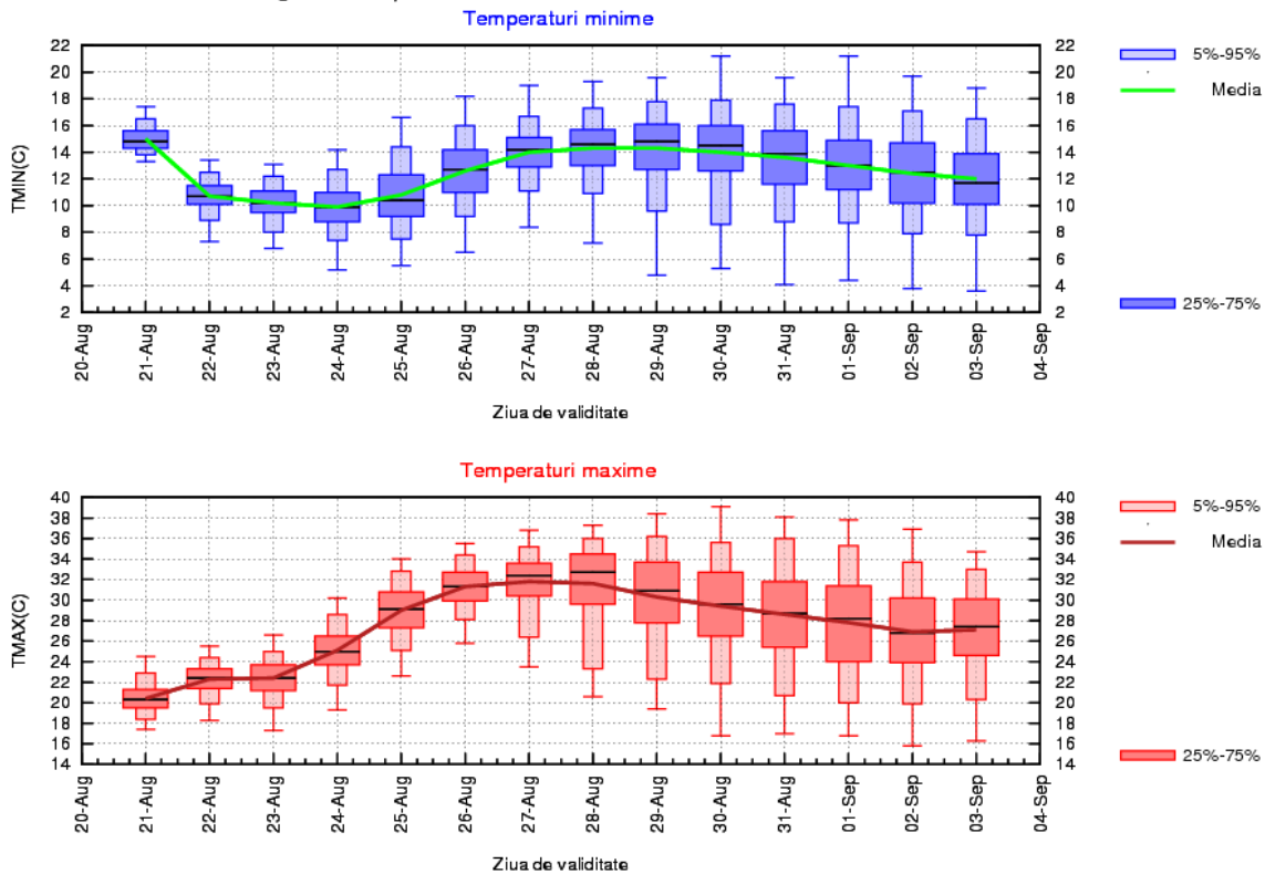
MARAMUREȘ Prognoza temperaturilor extreme. Model MOS-ECMWF-EPS. Baza:20170820 00 UTC
