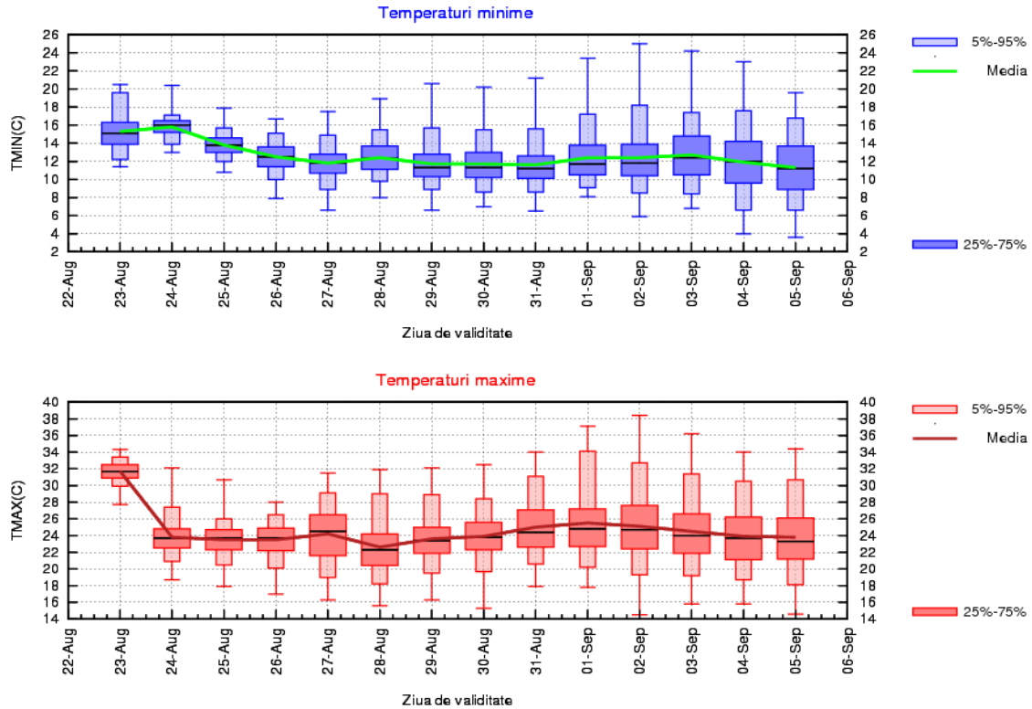
CRISANA Prognoza temperaturilor extreme. Model MOS-ECMWF-EPS. Baza:20210822 00 UTC
