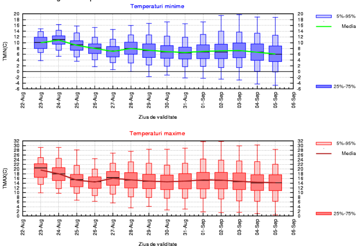
MUNTE Prognoza temperaturilor extreme. Model MOS-ECMWF-EPS. Baza:20210822 00 UTC
