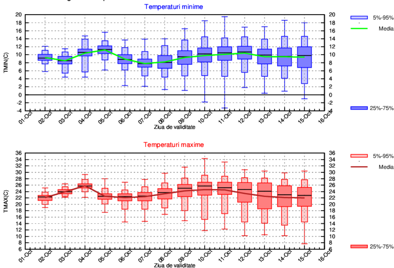
BANAT Prognoza temperaturilor extreme. Model MOS-ECMWF-EPS. Baza:20231001 00 UTC
