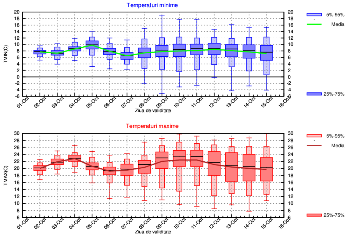
MARAMURES Prognoza temperaturilor extreme. Model MOS-ECMWF-EPS. Baza:20231001 00 UTC
