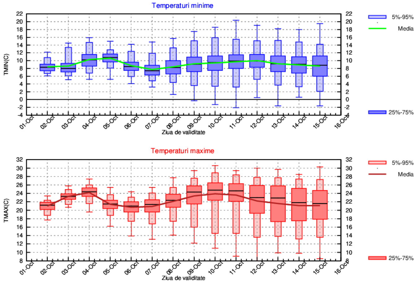
CRISANA Prognoza temperaturilor extreme. Model MOS-ECMWF-EPS. Baza:20231001 00 UTC
