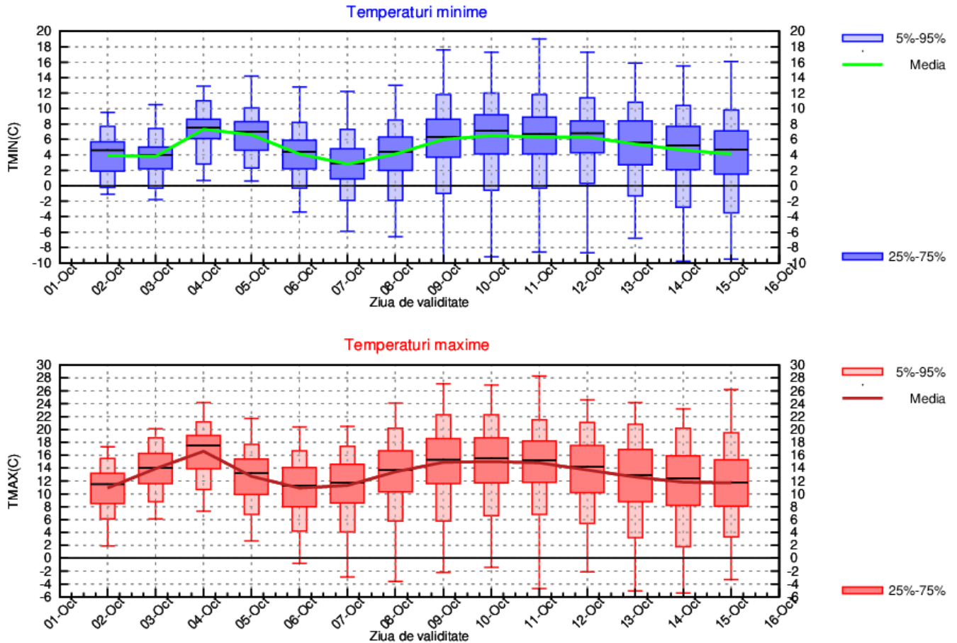
MUNTE Prognoza temperaturilor extreme. Model MOS-ECMWF-EPS. Baza:20231001 00 UTC
