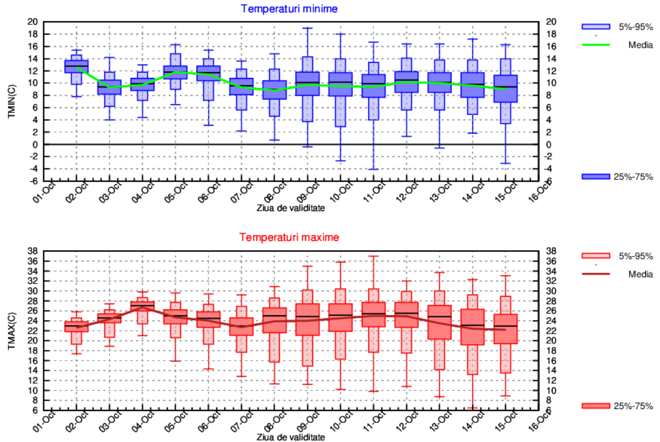
MUNTENIA Prognoza temperaturilor extreme. Model MOS-ECMWF-EPS. Baza:20231001 00 UTC
